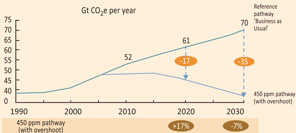
FIG 1.7 CARBON EMISSIONS PER YEAR: 1990–2030
